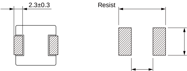
Land Pattern: [mm]
